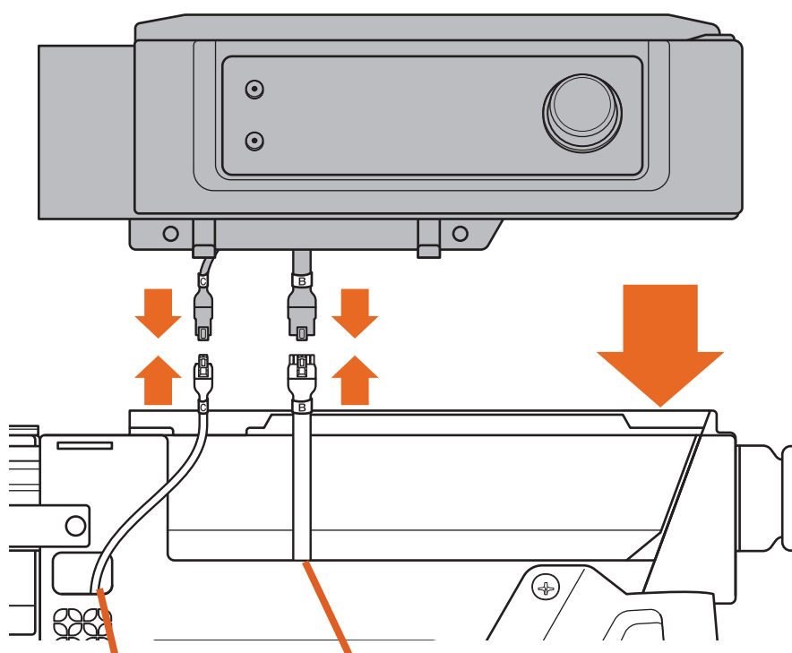
TEMPERATURE SENSOR 4-PIN CONNECTOR
